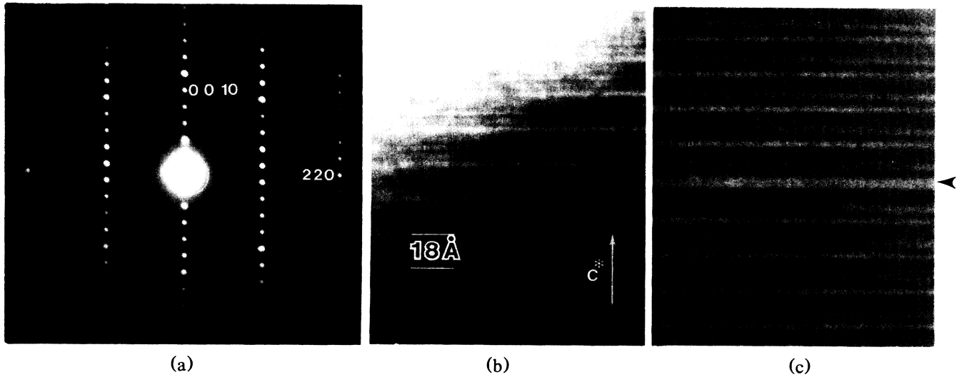
FIG. 2. (a) [1\bar{1}0] Selected-area electron diffraction pattern of 2223 superconductor. (b) The corresponding lattice image reveals a prominent 18-Å layering parallel to (001), similar to that of the bismuth 2122 superconductor (Refs. 9 and 14). (c) Defects in the layering (arrow) are relatively uncommon in the 2223 phase compared to the structurally related bismuth 2122 superconductor.
