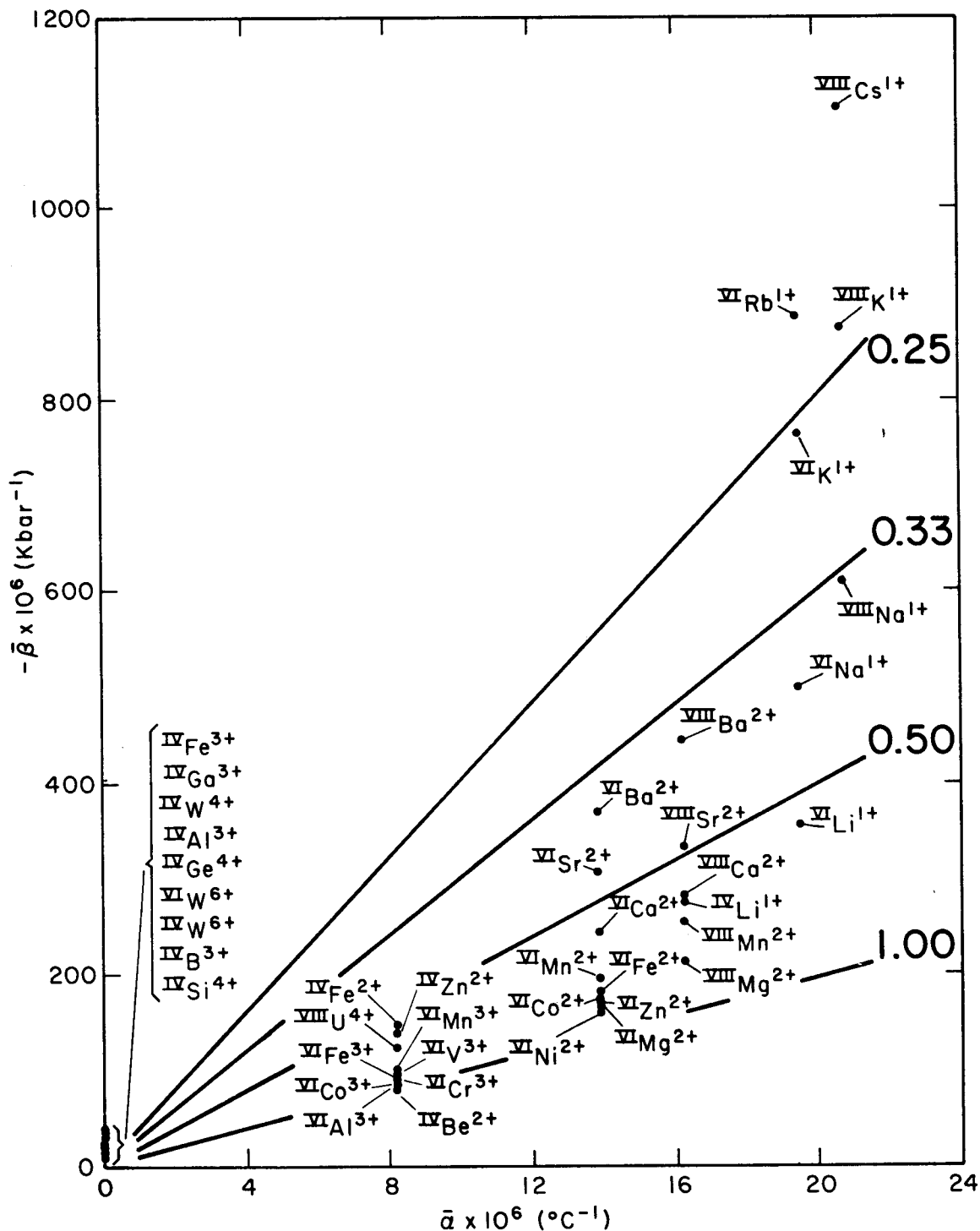
Fig. 4. Predicted values of \bar{\alpha}/\bar{\beta} for metal-oxygen bonds. Several lines of constant \bar{\alpha}/\bar{\beta} are drawn. If all the cation polyhedra in a given mineral fall near one such line, then the structural changes during cooling from high temperature will be the same as the structural changes during compression. Cations are given in the form ^p R^z , as described in Fig. 1.
