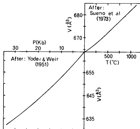
Fig. 1. Low albite unit-cell volume vs. temperature and pressure. The temperature and pressure axes have been scaled so that the slopes of the two portions of the graph appear similar. High-temperature data are from Sueno et al. (1973) and high-pressure data are from Yoder and Weir (1951).
